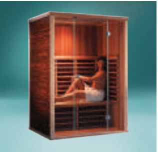
Platinum Series FIR Cabin Size: 150L x 120W x 190H cm, 2100W
